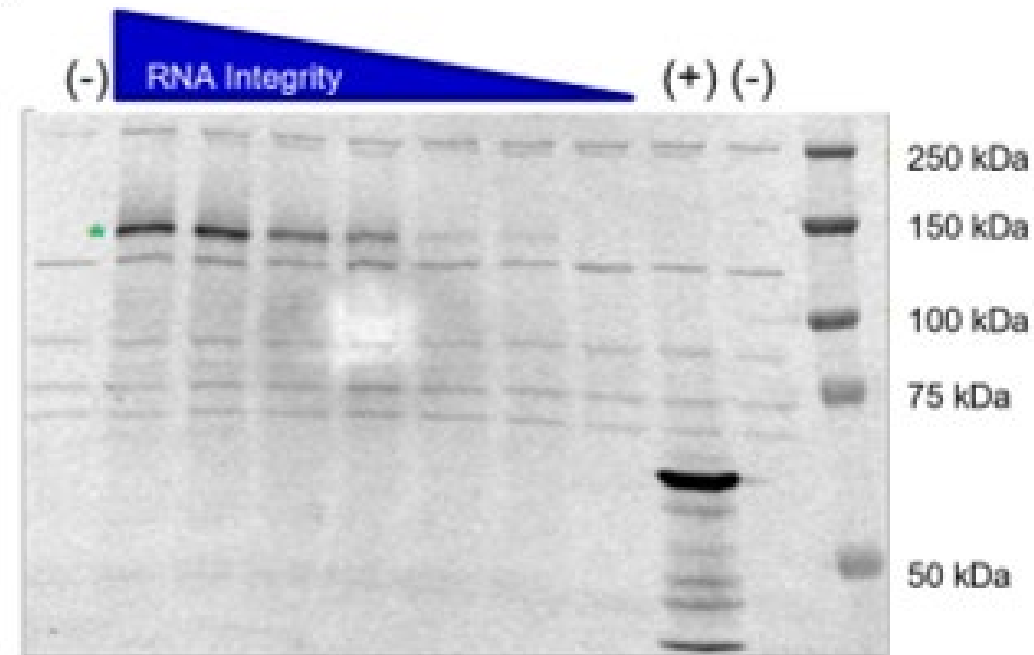
Fig. 6. Evaluation of translation from degraded mRNA species. (A) Full-length mRNA was thermally degraded to generate samples with diminishing levels of intact mRNA (and increased fragments). (B) Expression was evaluated in a cell-free expression system that incorporates a biotinylated lysine into newly translated proteins. SARS-CoV-2 spike protein expression is observed at the expected size for the non-glycosylated form (designated with a “*”) and at levels correlating with RNA integrity. No additional protein expression (i.e., truncated or off-target proteins) is observed beyond the species expressed in the negative control (-). “(+)” represents the positive control, “(-)” represents a negative control.
